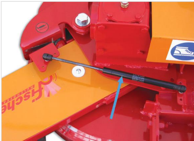
Heavy duty gas spring shocks on each swing arm
